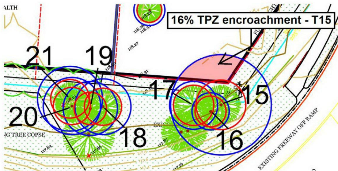
Figure 2: An excerpt of the current design, showing the proposed construction within the TPZ of Tree 15.
